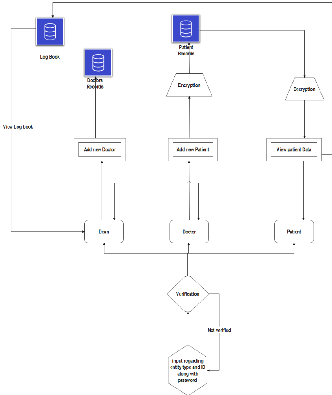
Figure 1 - Flowchart
