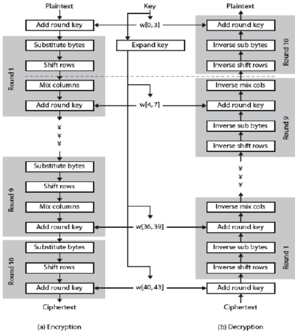
Figure 2 – AES Algorithm
