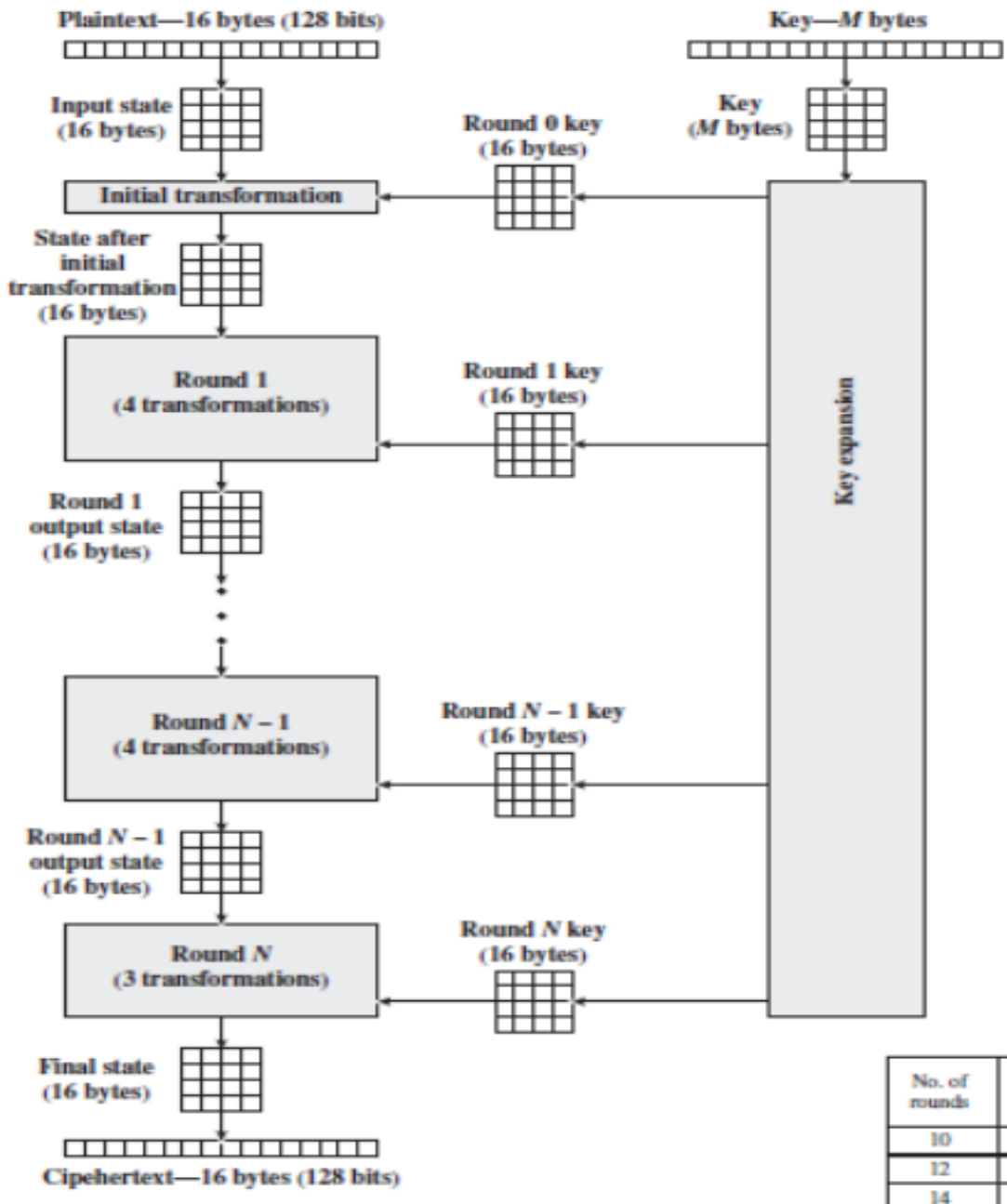
Figure 3 – AES Encryption
